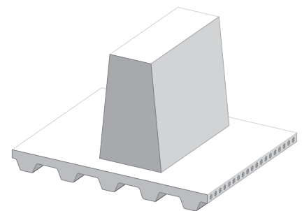
CAM 1010 (lwxh) Main dimensions [mm]: 12 x 23 x 18
