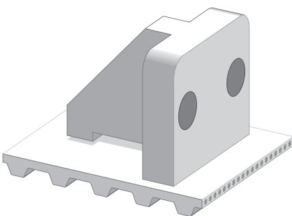
CAM 3003 (l x w x h) Main dimensions [mm]: 26 x 25 x 20
